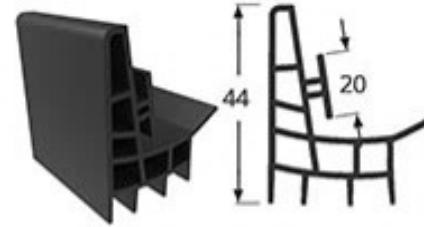
P240 PVC Gasket
